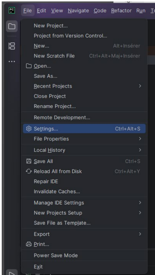
File / Settings
